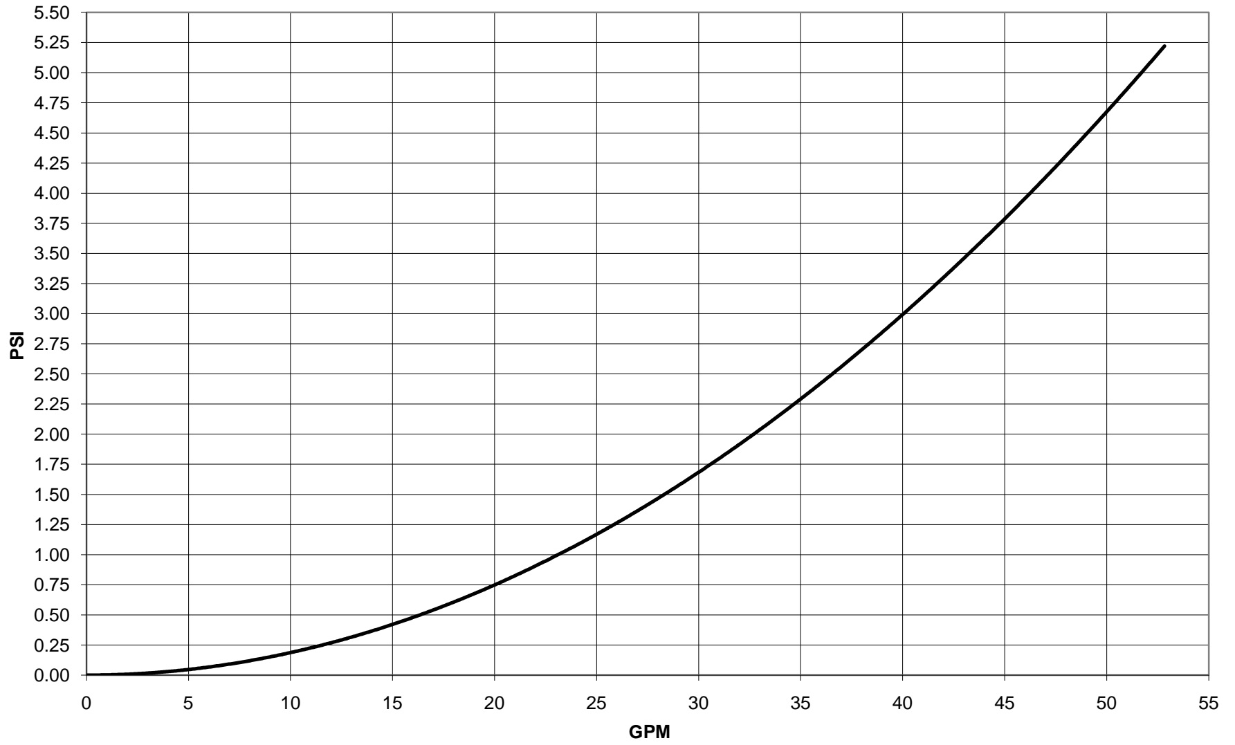
VFS 10-200 Pressure Drop
