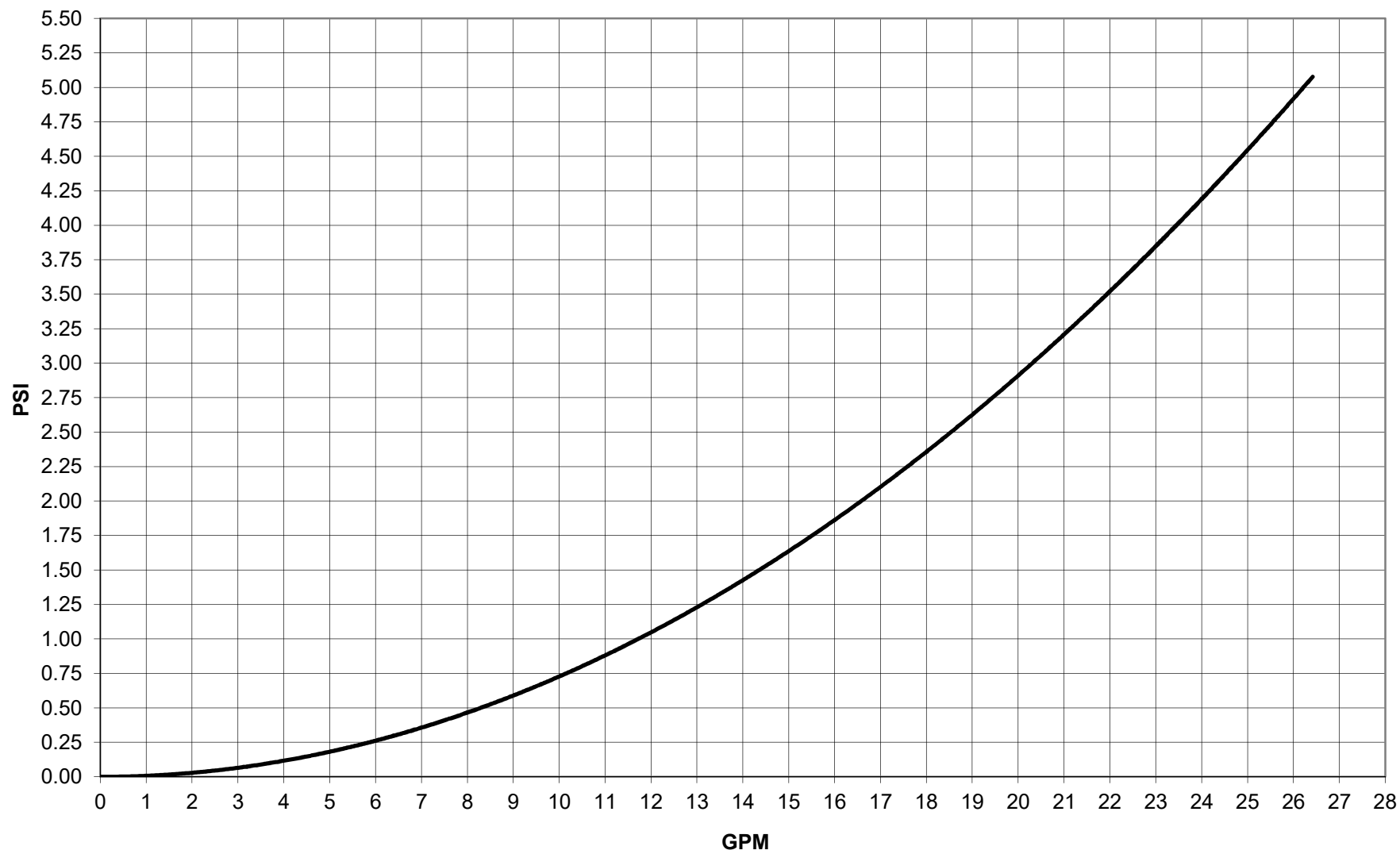
VFS 5-100 Pressure Drop
